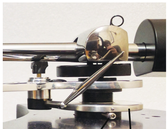
VTA CLAMPING GRUB SCREW
