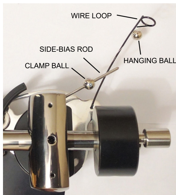
Photo showing side bias ball arrangement
