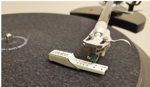
Photo of stylus force gauge to set tracking force
